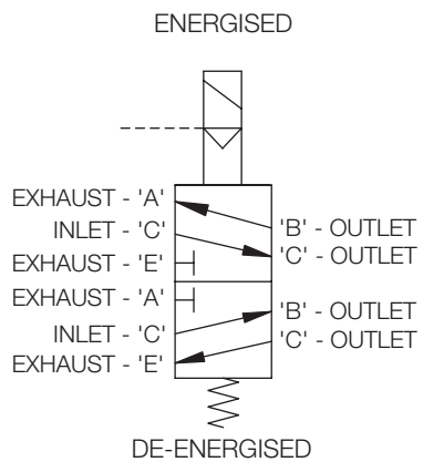
VALVE SYMBOL
